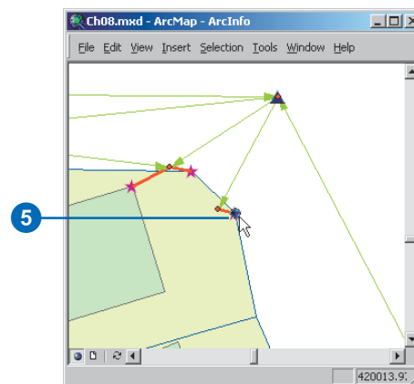
Unlinking survey points from feature vertices
