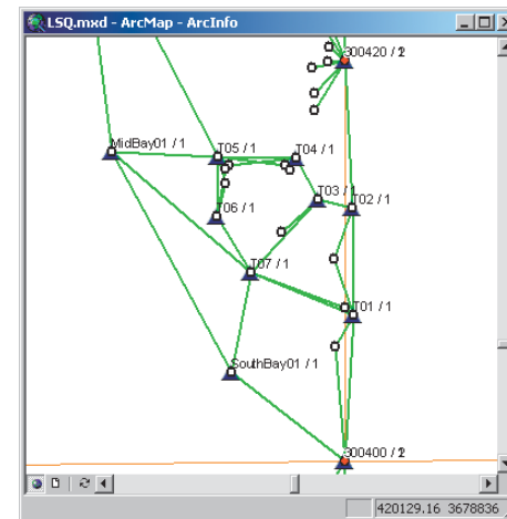
Least squares adjustment computation
