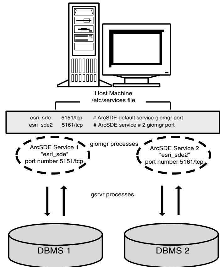
One host computer supporting two ArcSDE application servers
