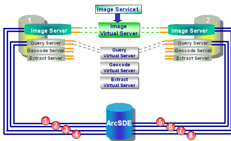
ArcSDE Connections Needed for One Image Service
