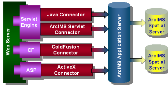
Business Logic Tier Components
